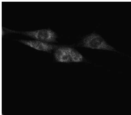
Figure 2. CSLM image of R3230AC cells treated with 2 \mu M TMR-Se for 1.5 h with excitation at 532 nm.
