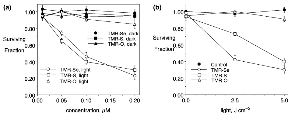
Figure 1. Effect of dyes TMR-O , TMR-S , and TMR-Se on the viability of R3230AC cells in culture in the dark or 24 h after exposure to (a) various concentrations of dye and 5.0 \text{ J cm}^{-2} of filtered 360–800 nm light or (b) 0.1 \mu\text{M} dye and variable light doses. Each point represents three separate experiments performed in duplicate for the viability of cultured R3230AC cells maintained in the dark or 24 h after exposure of cells to light. Data are expressed as the fraction of control cell viability, exposed to neither dyes nor light, error bars are the SEM.
