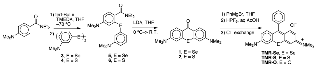
Scheme 1. Preparation of TMR-Se and TMR-S .
