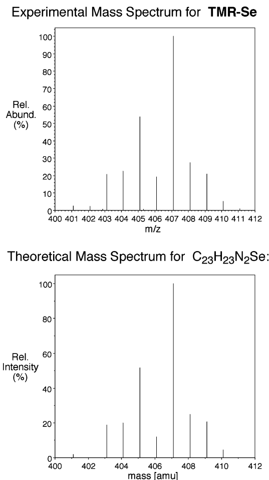
Figure 3. A comparison of the experimental mass spectrum of TMR-Se (top) with the theoretical mass spectrum of a molecule with the formula C 23 H 23 N 2 Se (bottom).
